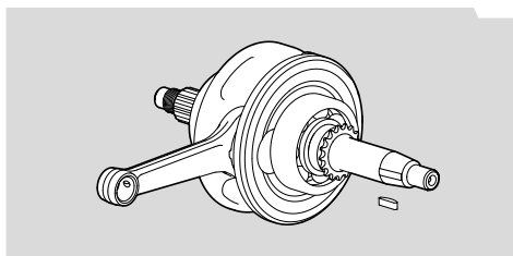
VILEBREQUIN CRANKSHAFT
